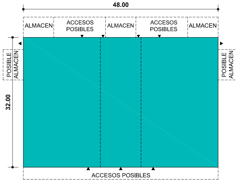
PABELLON POLIDEPORTIVO PB2 (32x48x7.5-9) 1536m 2
