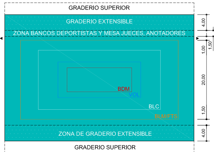
CAMPOS PRINCIPALES PB2 (32x48x7.5-9) 1536m 2
